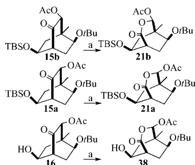
Scheme 8. Reagents and conditions: (a) 3 equiv. m -CPBA, 1.2 equiv. NaHCO 3 , CH 2 Cl 2 , 25 °C.
