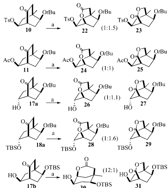
Scheme 5. Reagents and conditions: 3 equiv. m -CPBA, 1.2 equiv. NaHCO 3 , CH 2 Cl 2 , 25 °C.
