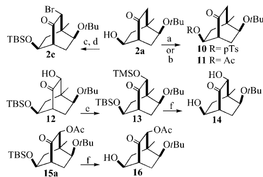
Scheme 3. (a) p -TsCl, py, DMAP, 0 °C to 25 °C; (b) Ac_2O , py, DMAP, 0 °C, 1 h 30 min; (c) TBSCl, DMF/imidazole, 0 °C to 25 °C, 16 h; (d) (i) TMSOTf, collidine, PhMe, 25 °C; (ii) NBS, THF, 0 °C; (e) TMS/imidazole, CH_2Cl_2 , 0 °C; (f) TBAF, THF, 0 °C.
