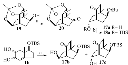
Scheme 4. (a) Dess–Martin periodinane, CH_2Cl_2 , py, 25 °C, 0.5 h; (b) TBSCl, DMF/imidazole, 0 °C to 25 °C, 16 h; (c) 2.4 equiv. Pb(OAc)_4 , PhMe then K_2CO_3/MeOH, H_2O , 25 °C.
