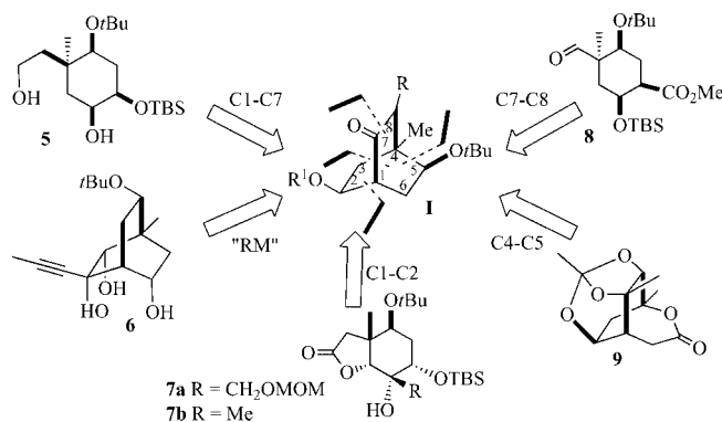
Scheme 2. Routes for practical syntheses of stereopure six-membered ring subunits by applying suitable reaction sequences to conveniently functionalized domino product I .
