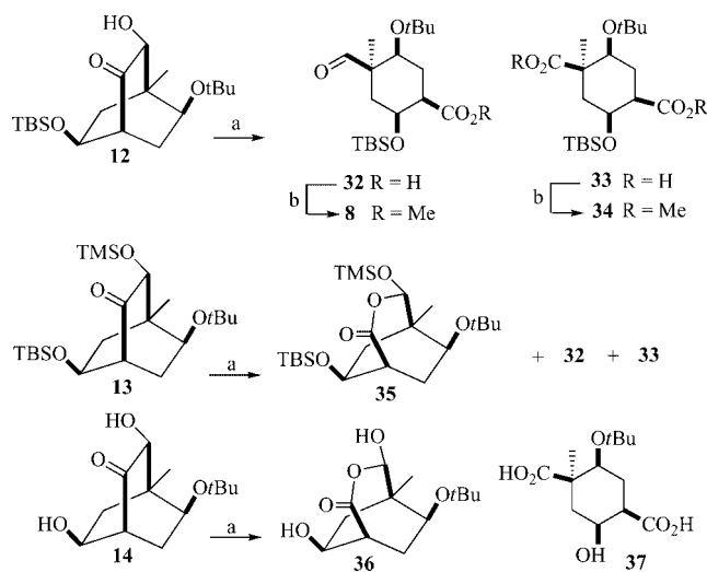
Scheme 7. Reagents and conditions: (a) 3 equiv. m -CPBA, 1.2 equiv. NaHCO 3 , CH 2 Cl 2 , 25 °C. (b) TMSCHN 2 , Et 2 O, MeOH, 0 °C to 25 °C.
