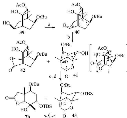
Scheme 10. (a) Dess–Martin periodinane, \text{CH}_2\text{Cl}_2 , 25 °C; (b) 3 equiv. m -CPBA, 1.2 equiv. \text{NaHCO}_3 , \text{CH}_2\text{Cl}_2 , 25 °C, 20 h; (c) TBSCl, DMF/imidazole, 0 °C to 25 °C, 16 h; (d) \text{K}_2\text{CO}_3 , MeOH/ \text{H}_2\text{O} , 25 °C.
